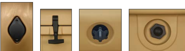
Bluetooth Temp Sensor Latch Drain Valve Pressure Relief Valve
